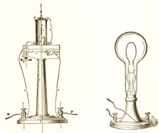
Edison's Platinum Lamp on Carbon Support, 1879.
