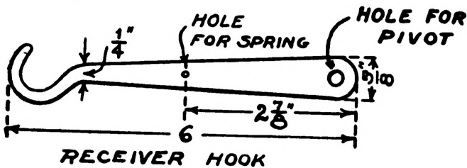
FIG. 95.—Details of the Receiver Hook.
