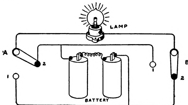
FIG. 161.—Double Control System.
