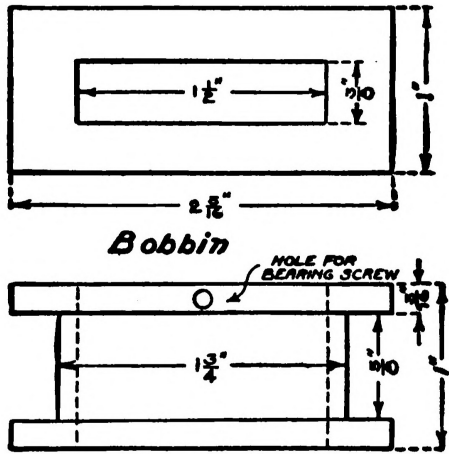
FIG. 68.—Details of the Bobbin.
