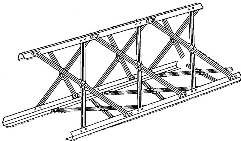
Fig. 17. Trellis Type of Aluminum Girder used in Longitudinals of Zeppelin Frame
