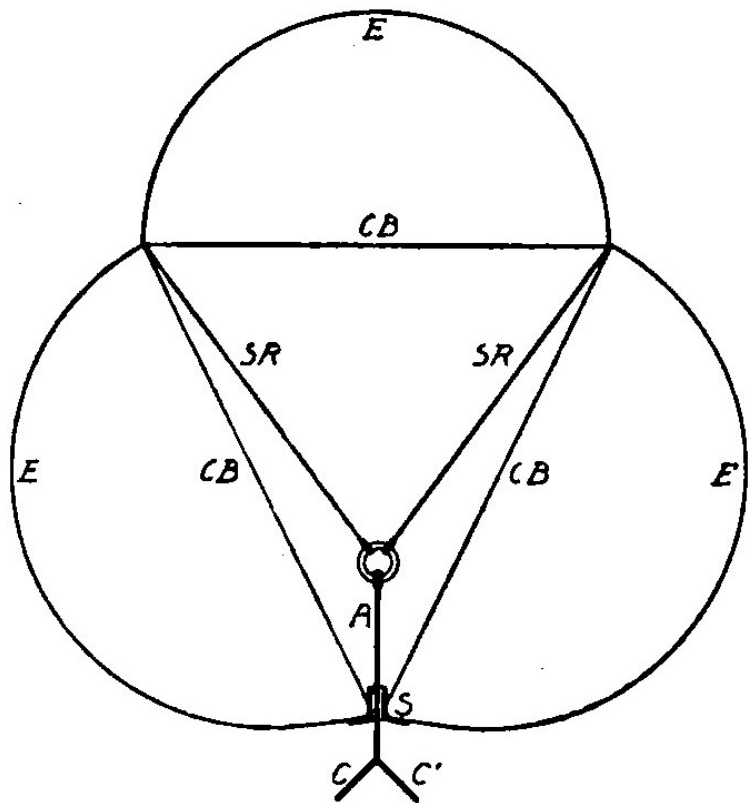
Fig. 14. Section of Astra-Torres, Illustrating Method of Suspension. CB, Bracing of Heavy Fabric Bands; SR and A, Suspension Ropes and Cable Passing through Envelope; S, Expansion Sleeve in Envelope; CC', Ropes to Sides of Car; E, Envelope
