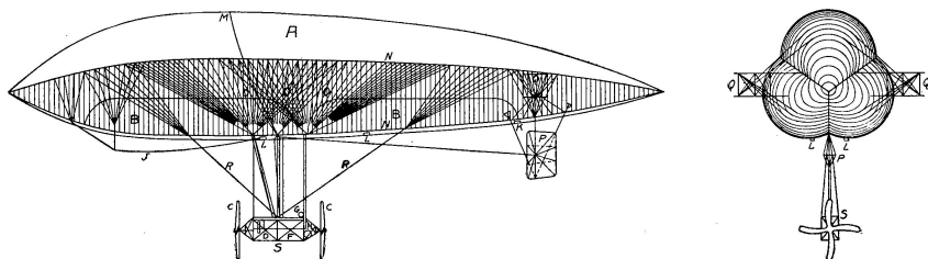
Fig. 21. Side and End Views of British Astra-Torres Dirigible Used for Anti-Submarine Patrol Service
