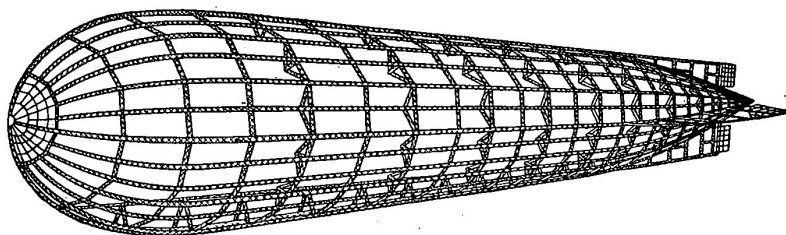
Fig. 18. Aluminum Frame Construction of Zeppelin Hull
