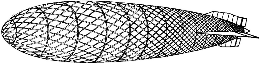
Fig. 19. Schutte-Lanz Type of Frame Construction of Laminated Wood with Aluminum Fittings
