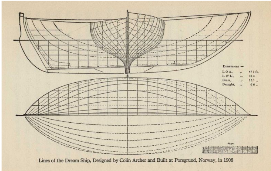
Lines of the Dream Ship, Designed by Colin Archer and Built at Porsgrund, Norway, in 1908
