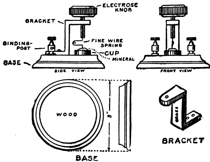
Fig. 211.—Details of the Crystal Detector.
