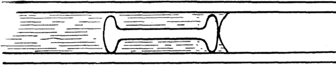
FIG. 2.—Column and index of minimum thermometer.
